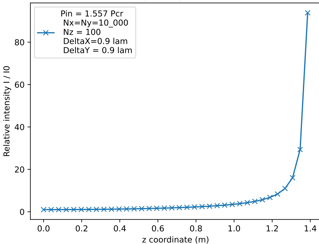
Relative intensity at x, y = 0 vs. z coordinate
